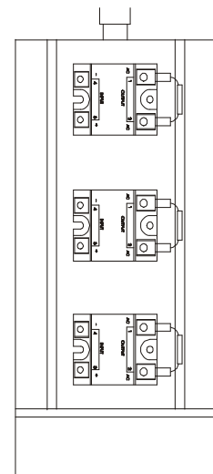
H x W x D = 304 x 125 x 181 mm Slot = 110 mm for M5 bolt
