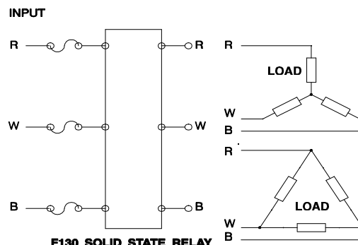
F130 SOLID STATE RELAY
