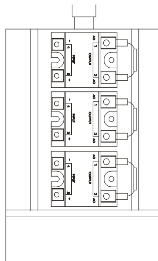
H x W x D = 219 x 125 x 181 mm Slot = 110 mm for M5 bolt
