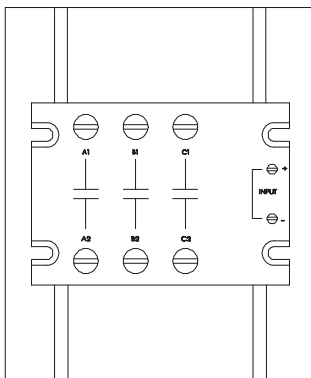
H x W x D = 150 x 125 x 155 mm Slot = 110 mm for M5 bolt
