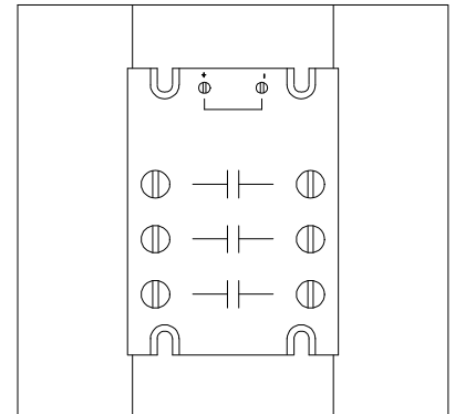
H x W x D = 150 x 150 x 93 mm Slot = 134 mm for M6 bolt
